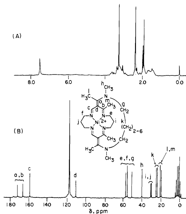
Figure 3. (A) Proton NMR spectrum of [\text{Ni}((\text{CH}_2)_6(\text{MeNEthi})_2\text{Me}_2\text{-}[16]\text{tetraeneN}_4)](\text{PF}_6)_2 . (B) Carbon-13 NMR spectrum of [\text{Ni}((\text{CH}_2)_6(\text{MeNEthi})_2\text{Me}_2\text{-}[16]\text{tetraeneN}_4)](\text{PF}_6)_2 .
