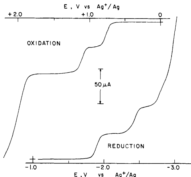
Figure 4. Voltammogram for [Ni((CH 2 ) 6 (MeNEthi) 2 Me 2 [16]tetraeneN 4 )](PF 6 ) 2 in 0.1 N n -Bu 4 NBF 4 in CH 3 CN; Ag/AgNO 3 (0.1 N) as the reference electrode.
