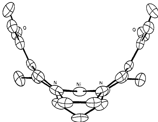
Figure 2. Crystal structure of the precursor complex [\text{Ni}((\text{MeOEt})_2\text{Me}_2[15]\text{tetraeneN}_4)](\text{ClO}_4)_2 .
