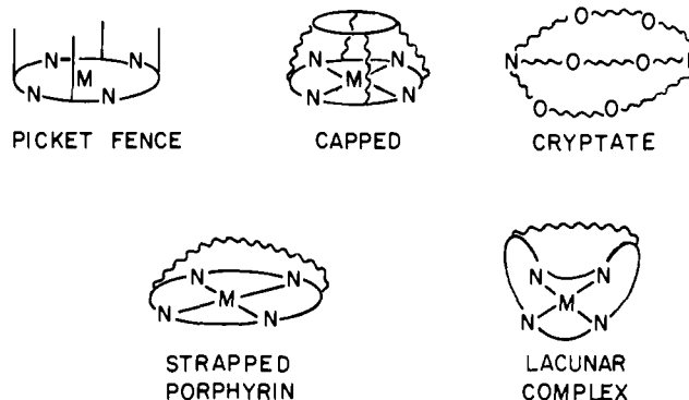
Figure 1. Diagrammatic representation of the fixed (smooth lines) and flexible (wavy lines) components of molecular species having permanent voids.
